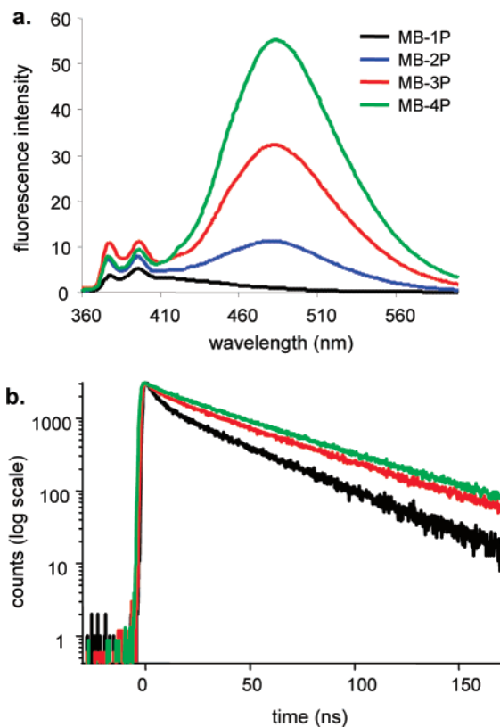
Figure 5. (a) Steady-state emission spectra of MB-1P (black), MB-2P (blue), MB-3P (red), and MB-4P (green) with excess cDNA in buffer. (b) Fluorescence decay of MB-2P (black), MB-3P (red), and MB-4P (green) at 480 nm. [MB] = 200 nM, [cDNA] = 2 \mu M.
