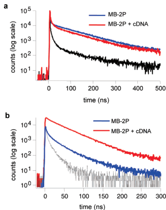
Figure 2. Fluorescence decay traces after 337 nm excitation of 1 μM MB-2P (blue) and MB-2P with target DNA (red) in buffer solution. Fluorescence emissions were monitored at (a) the pyrene monomer wavelength (398 nm) and at (b) the pyrene excimer wavelength (480 nm).
